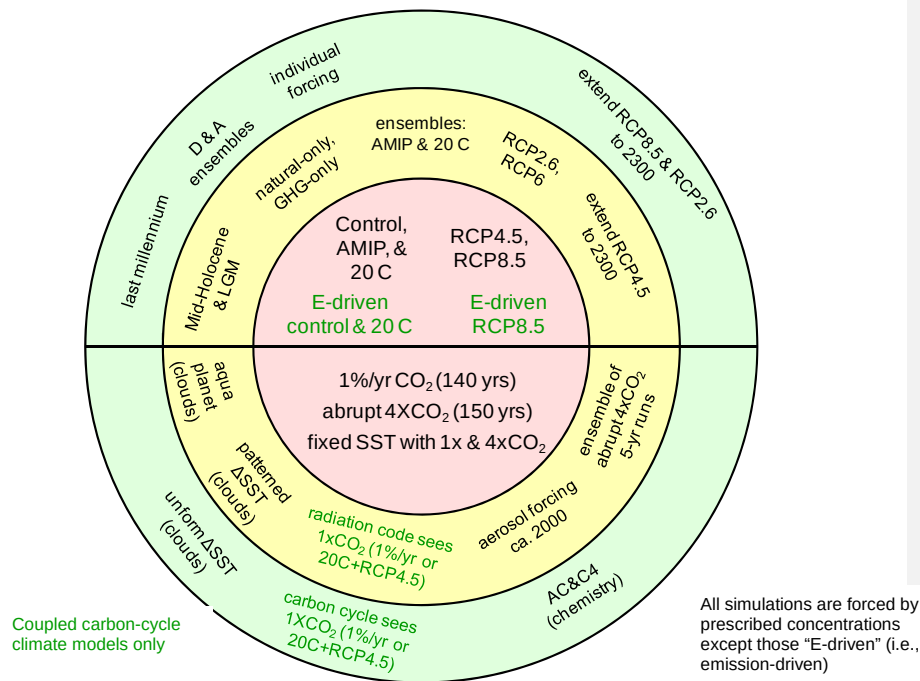
Figure 3: Schematic summary of CMIP5 long-term experiments.
